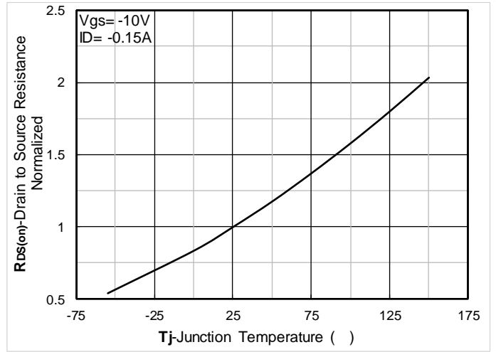
Figure8. Normalized On-Resistance
